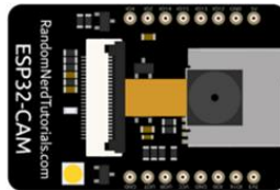
Gambar 2. 3 Esp 32 Cam
