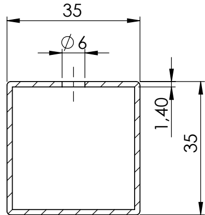
SECTION S-S SCALE 1 : 1
